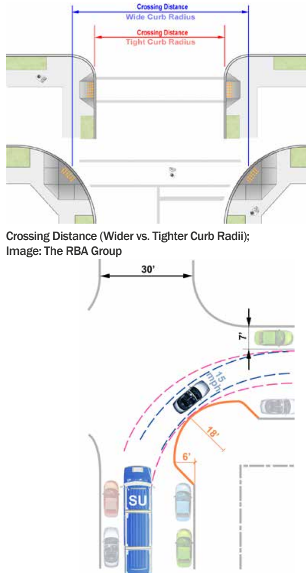
Single Unit (SU) Truck Turning Radii vs. Personal Car Turning Radii. Image: The RBA Group
