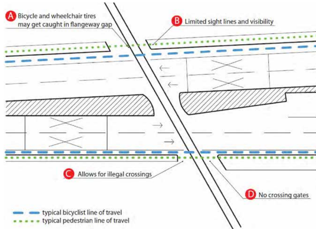
Graphic: Caltrans, Complete Intersections: A Guide to Reconstructing Intersections and Interchanges for Bicyclists and Pedestrians
